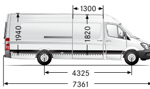
Extra-long with 4325 mm wheelbase and rear overhang of 2015 mm, high roof
