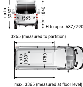
Medium with 3665 mm wheelbase, super-high roof
