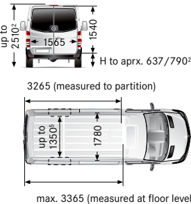
Medium with 3665 mm wheelbase, standard roof
