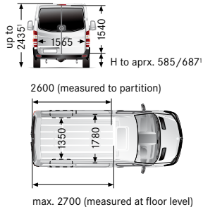
Short with 3250 mm wheelbase, standard roof
