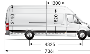
Extra-long with 4325 mm wheelbase and rear overhang of 2015 mm, super-high roof
