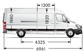
Long with 4325 mm wheelbase, high roof
