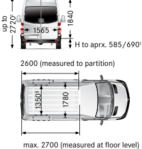
Short with 3250 mm wheelbase, high roof
