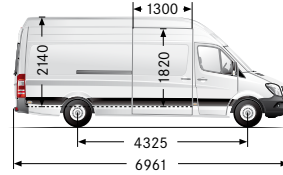
Long with 4325 mm wheelbase, super-high roof
