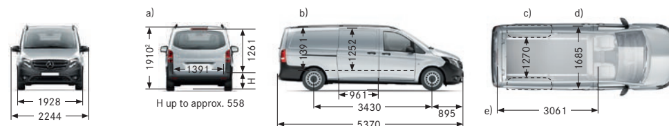
Extra-long panel van with 3430mm wheelbase
