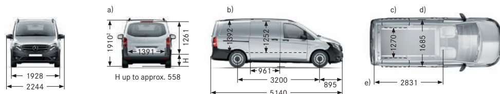
Long panel van with 3200mm wheelbase
