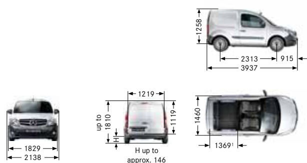
Compact panel van with 2313 mm wheelbase
